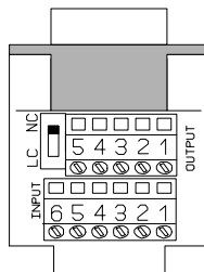
Figure 1 – Connector view (IB-ADP adapter)
