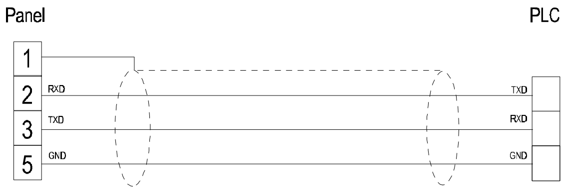
Figure 1. Cable diagram
