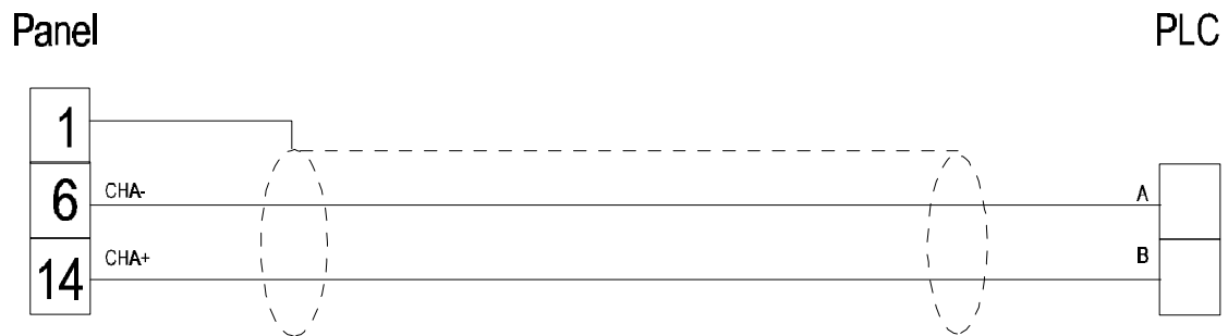
Figure 1. Cable diagram
