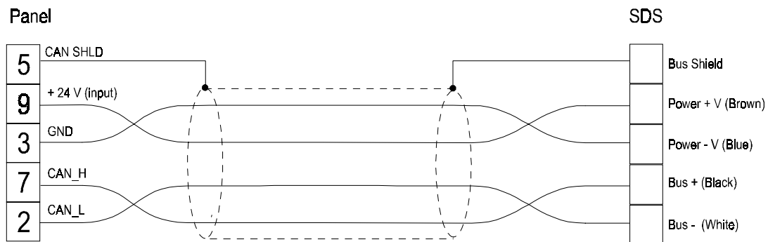
Figure 1. Cable diagram
