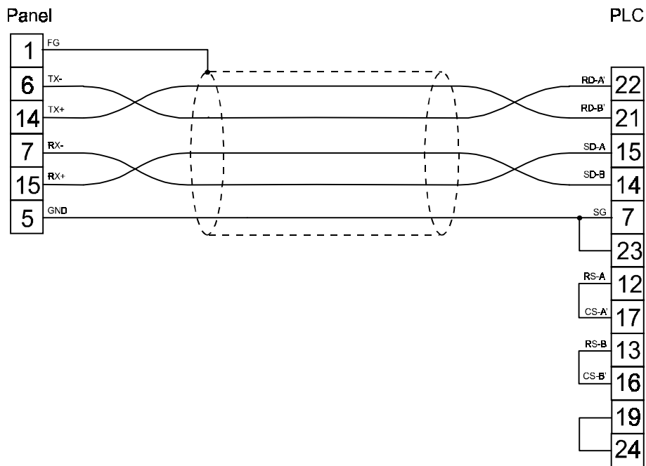
figure 1. Cable diagram
