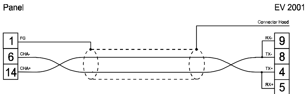
figure 1. Cable diagram
