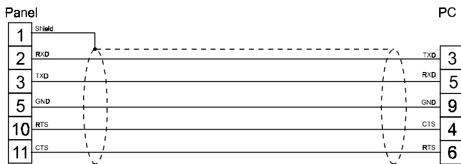
figure 1. Cable diagram
