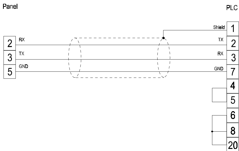
figure 1. Cable diagram
