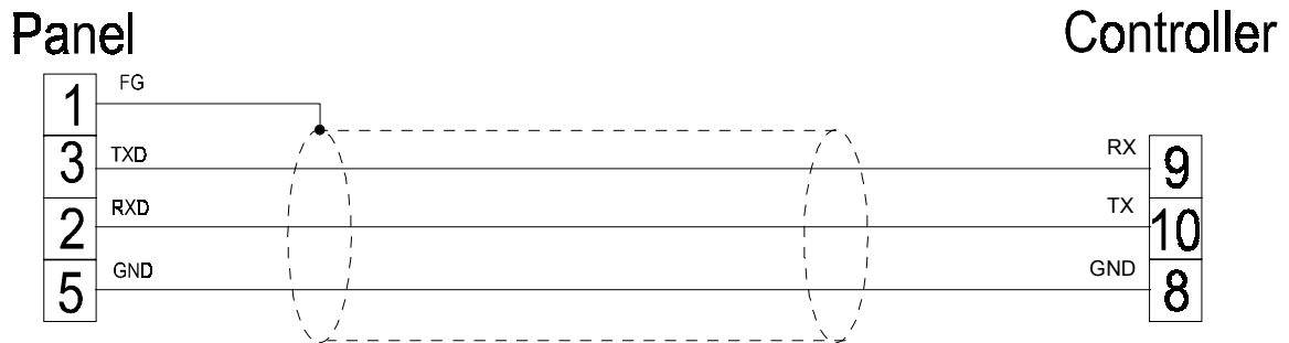
Figure 1. Cable diagram
