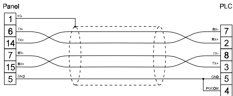
figure 1. Cable diagram
