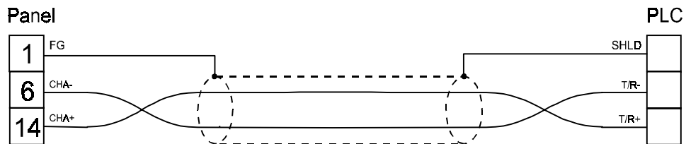
figure 1. Cable diagram
