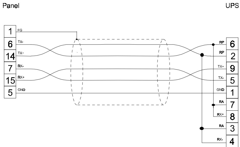
figure 1. Cable diagram
