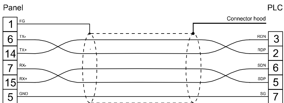
Figure 1. Cable diagram
