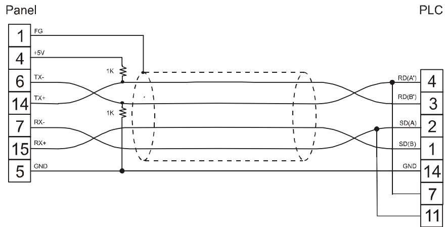
figure 1. Cable diagram
