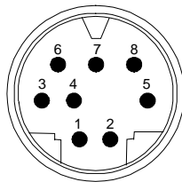
Connector Front View (Pin Side)
