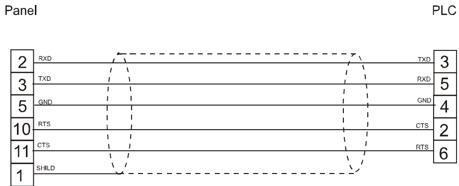
figure 1. Cable diagram
