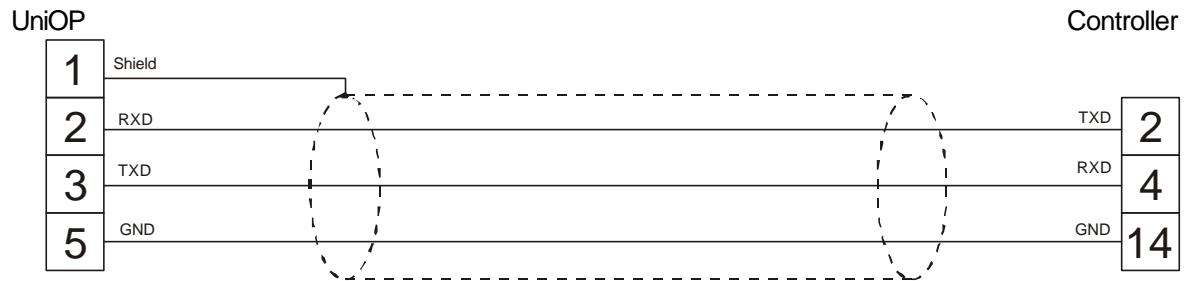
figure 1. Cable diagram
