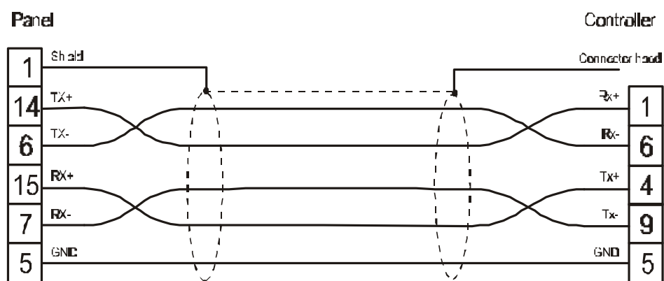
Figure 1. Cable diagram
