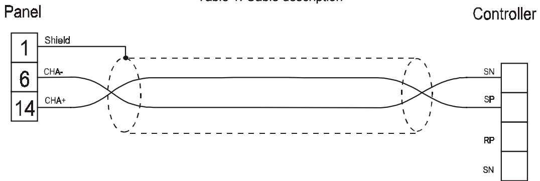
Figure 1. Cable diagram
