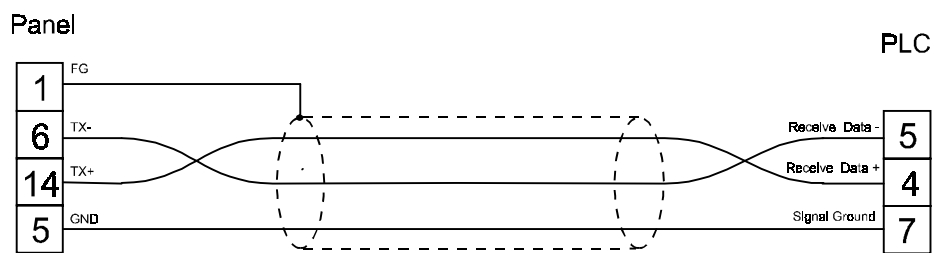
figure 1. Cable diagram
