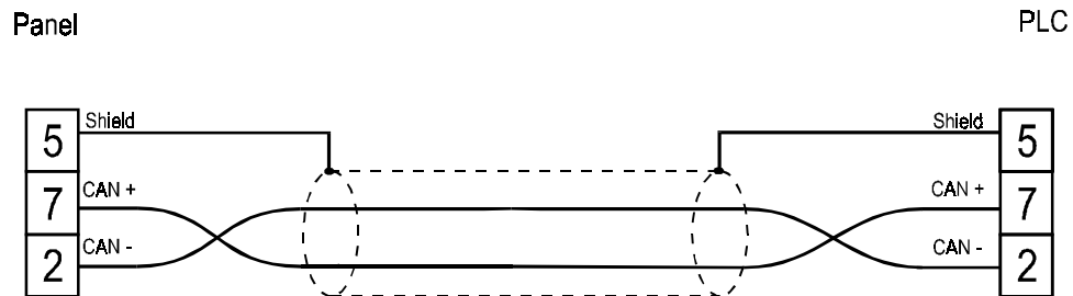
Figure 1. Cable diagram
