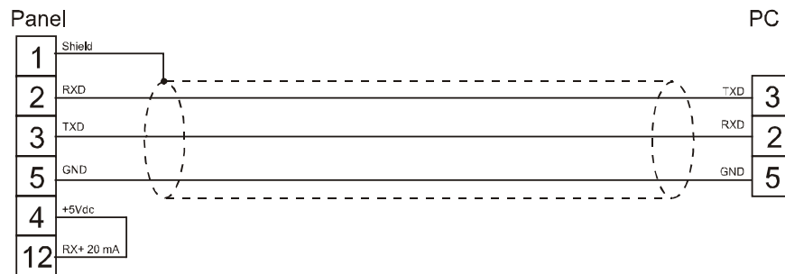
figure 1. Cable diagram
