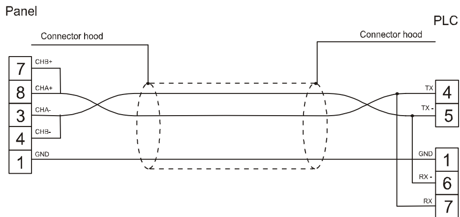
Figure 1. Cable diagram
