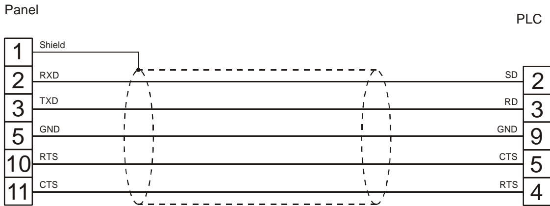
figure 1. Cable diagram
