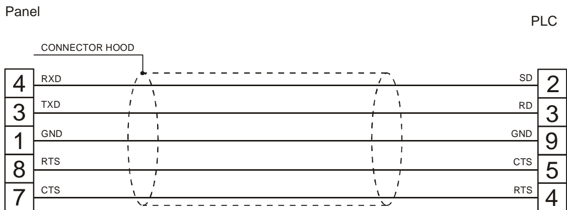
figure 1. Cable diagram
