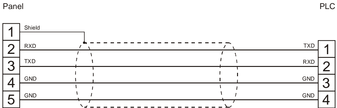
Figure 1. Cable diagram
