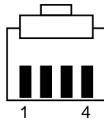
Figure 2. PLC Connector (front view)
