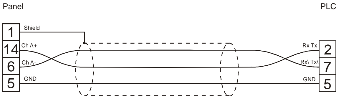
Figure 1. Cable diagram
