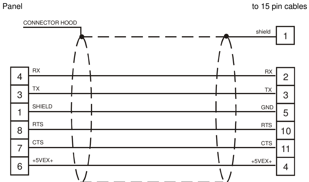
figure 1. Cable diagram
