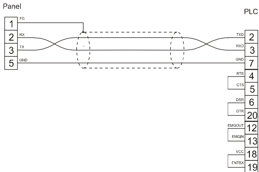
figure 1. Cable diagram
