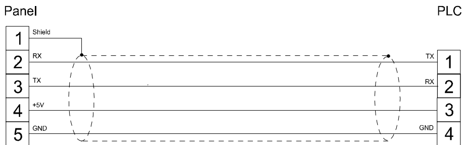
figure 1. Cable diagram
