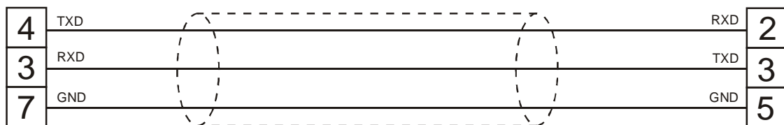
figure 1. Cable diagram
