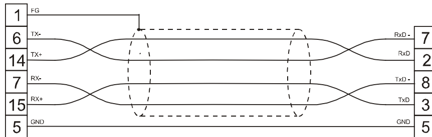
figure 1. Cable diagram
