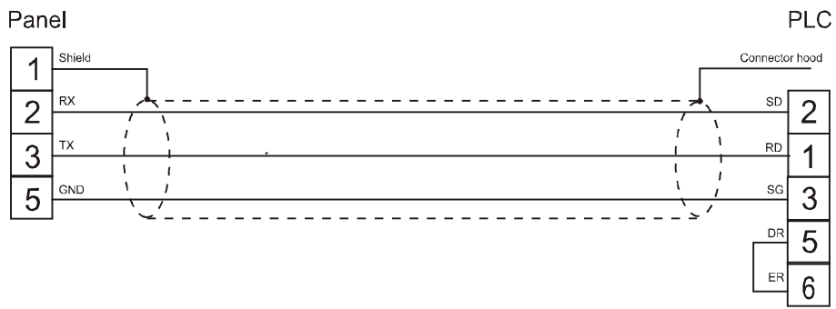
Figure 1. Cable diagram
