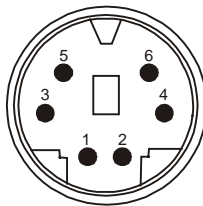
Figure 2. PLC connector (pin side)
