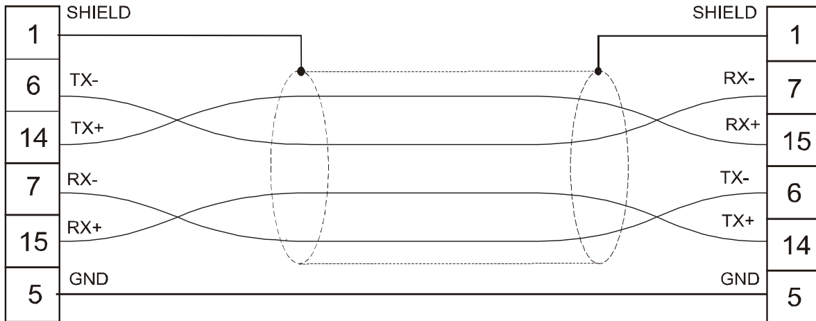
figure 1. Cable diagram
