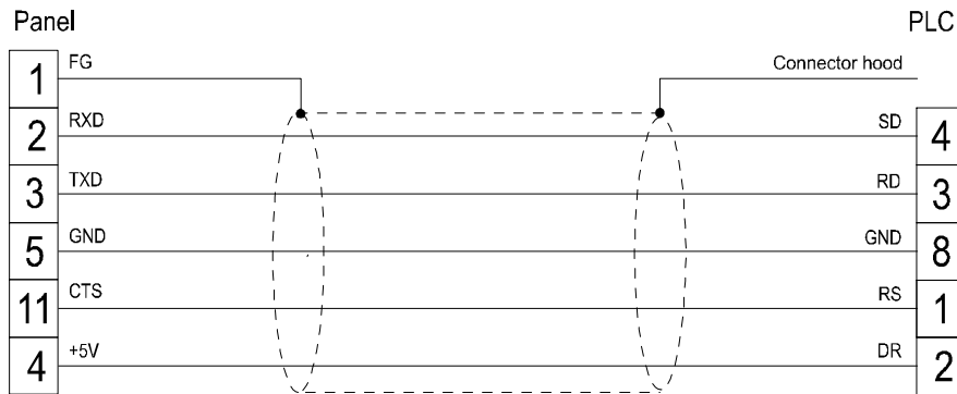
Figure 1. Cable diagram
