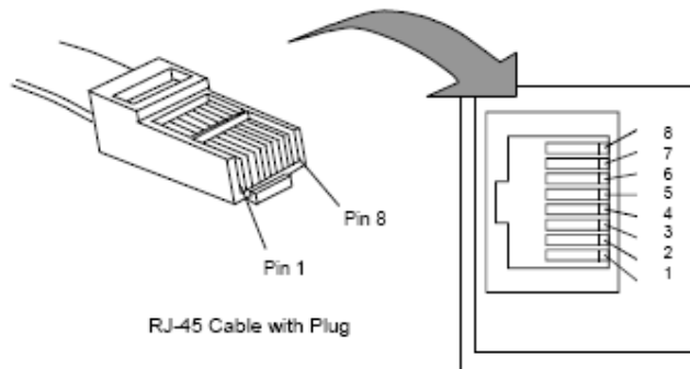
Figure 2. PLC connector
