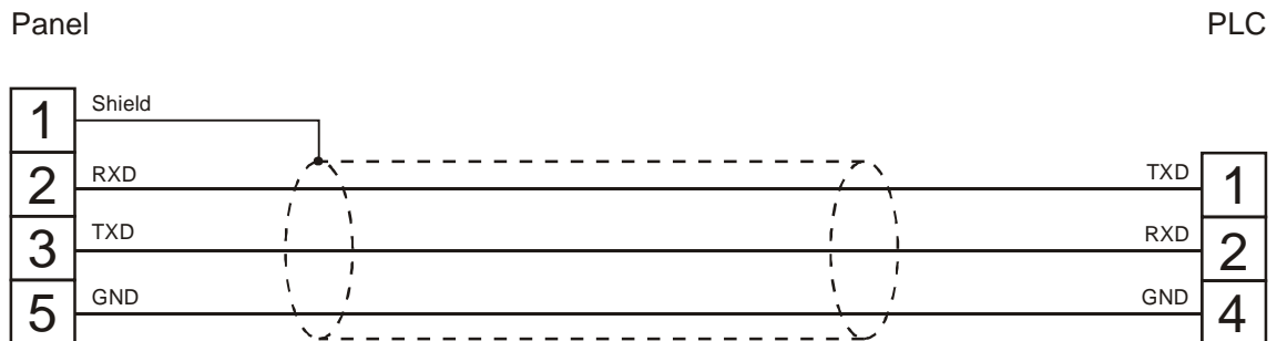
Figure 1. Cable diagram
