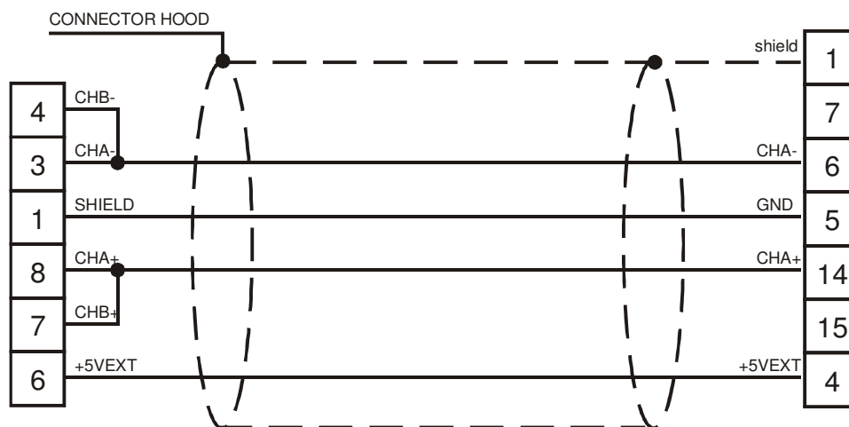
Figure 1. Cable diagram
