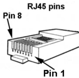
Figure 2. PLC connector
