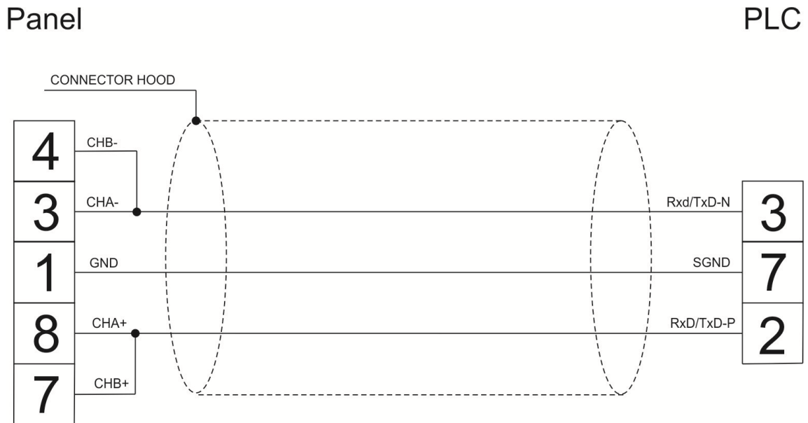
Figure 1. Cable diagram
