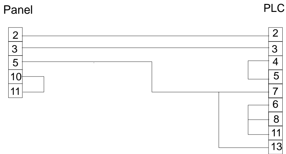
Figure 1. Cable diagram
