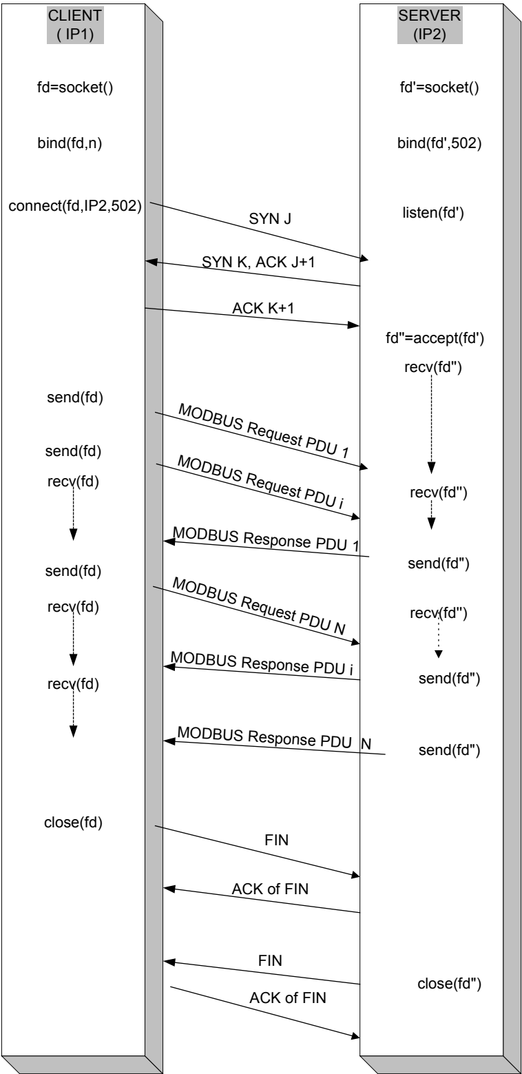
Figure 9: MODBUS Exchanges
